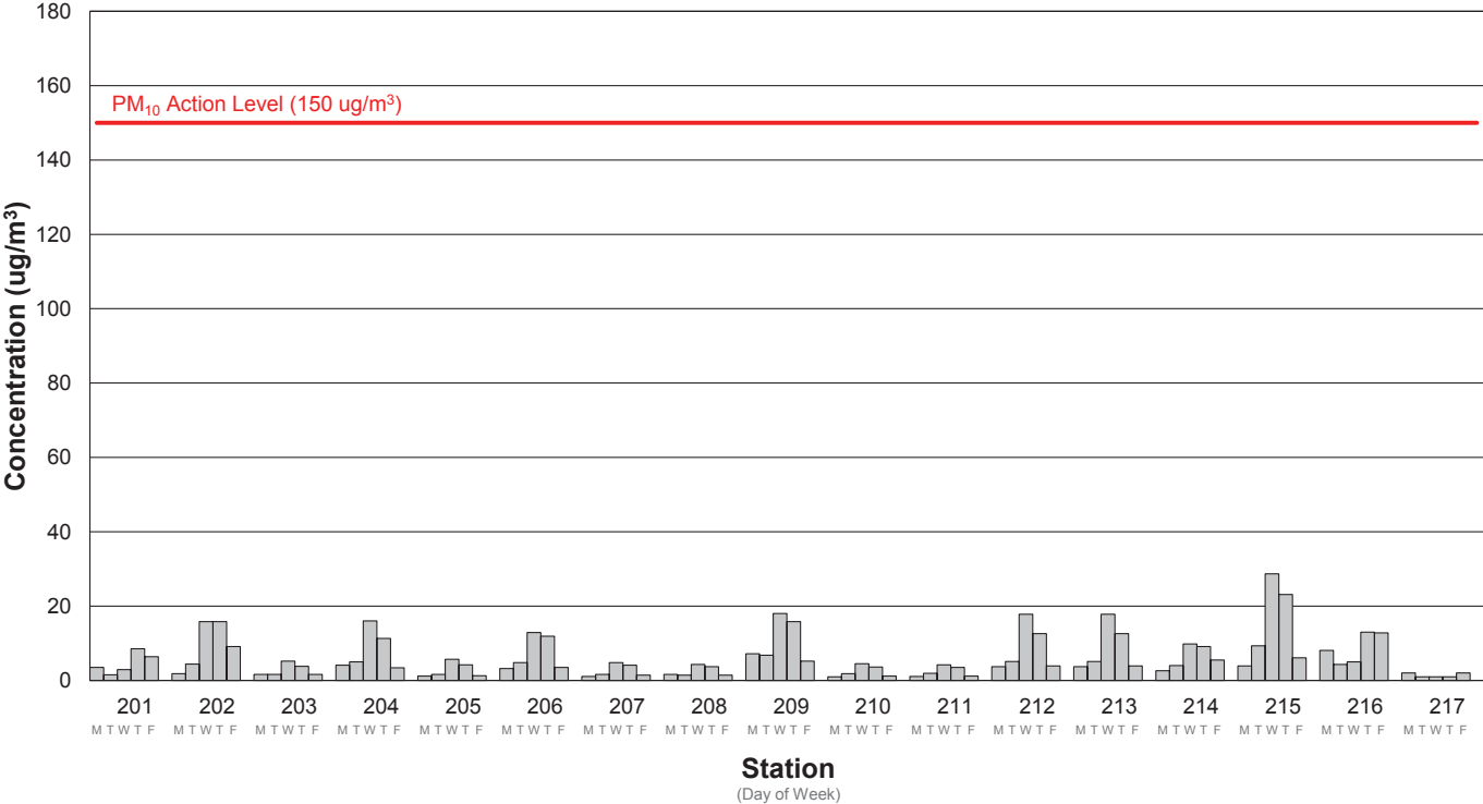
Average PM10 Concentration Week 90: 3/2/2026 - 3/6/2026
