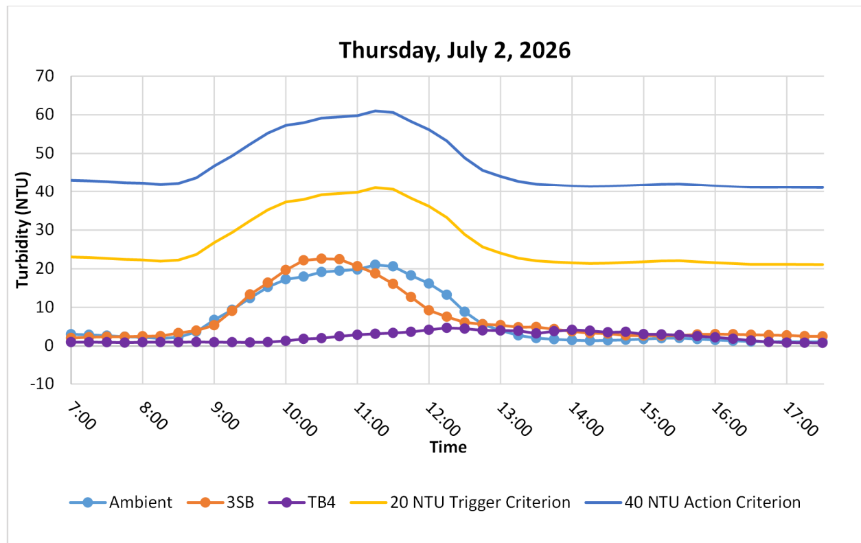
Figure 6. Hourly rolling average turbidity readings from 07:00 to 17:30.
