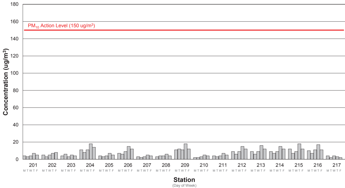
Average PM10 Concentration Week 107: 6/29/2026 - 7/3/2026
