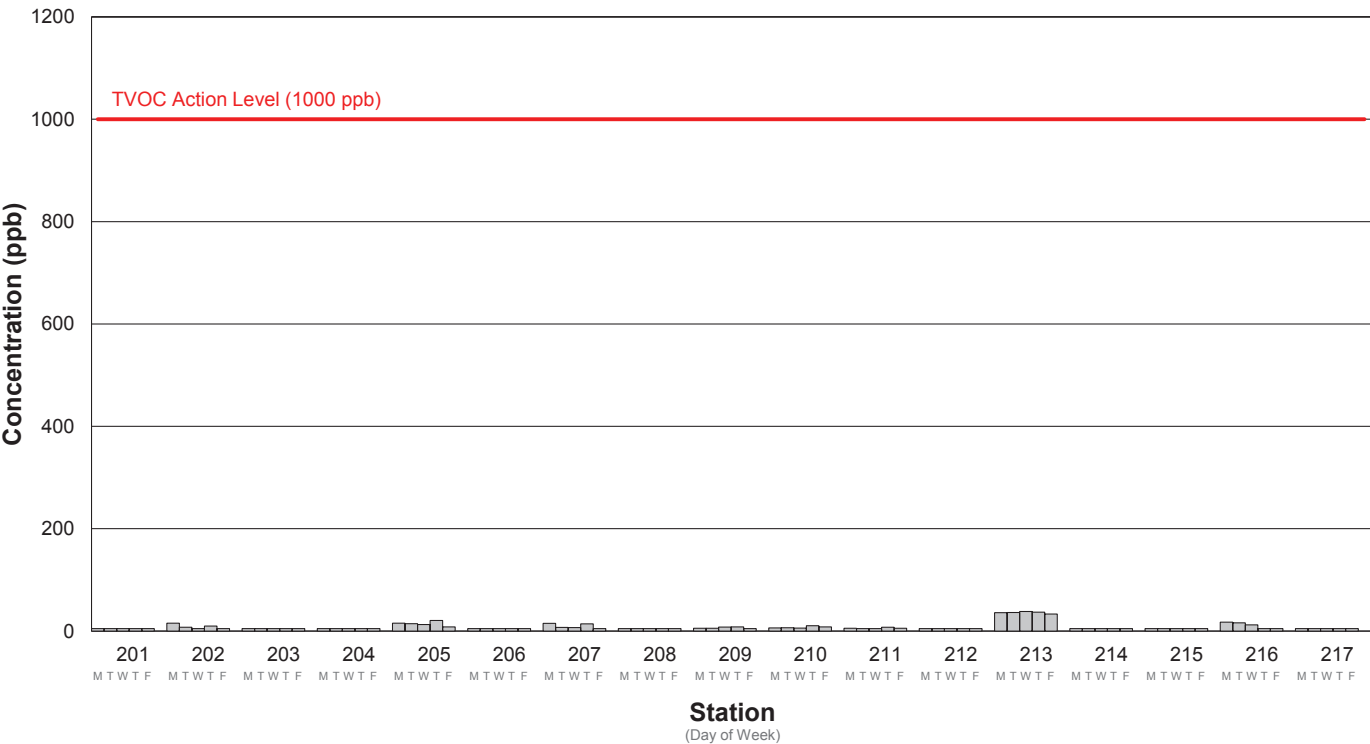
Average TVOC Concentration Week 107: 6/29/2026 - 7/3/2026
