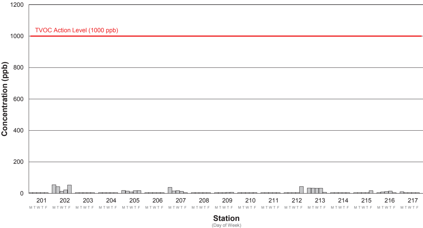
Average TVOC Concentration Week 108: 7/6/2026 - 7/10/2026
