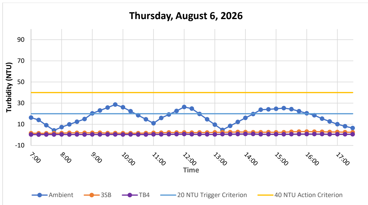
Figure 6. Hourly rolling average turbidity readings from 07:00 to 17:30
