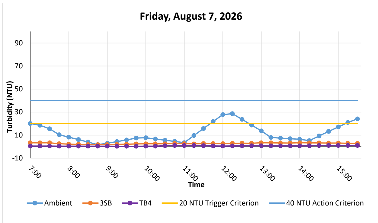
Figure 7. Hourly rolling average turbidity readings from 07:00 to 15:30
