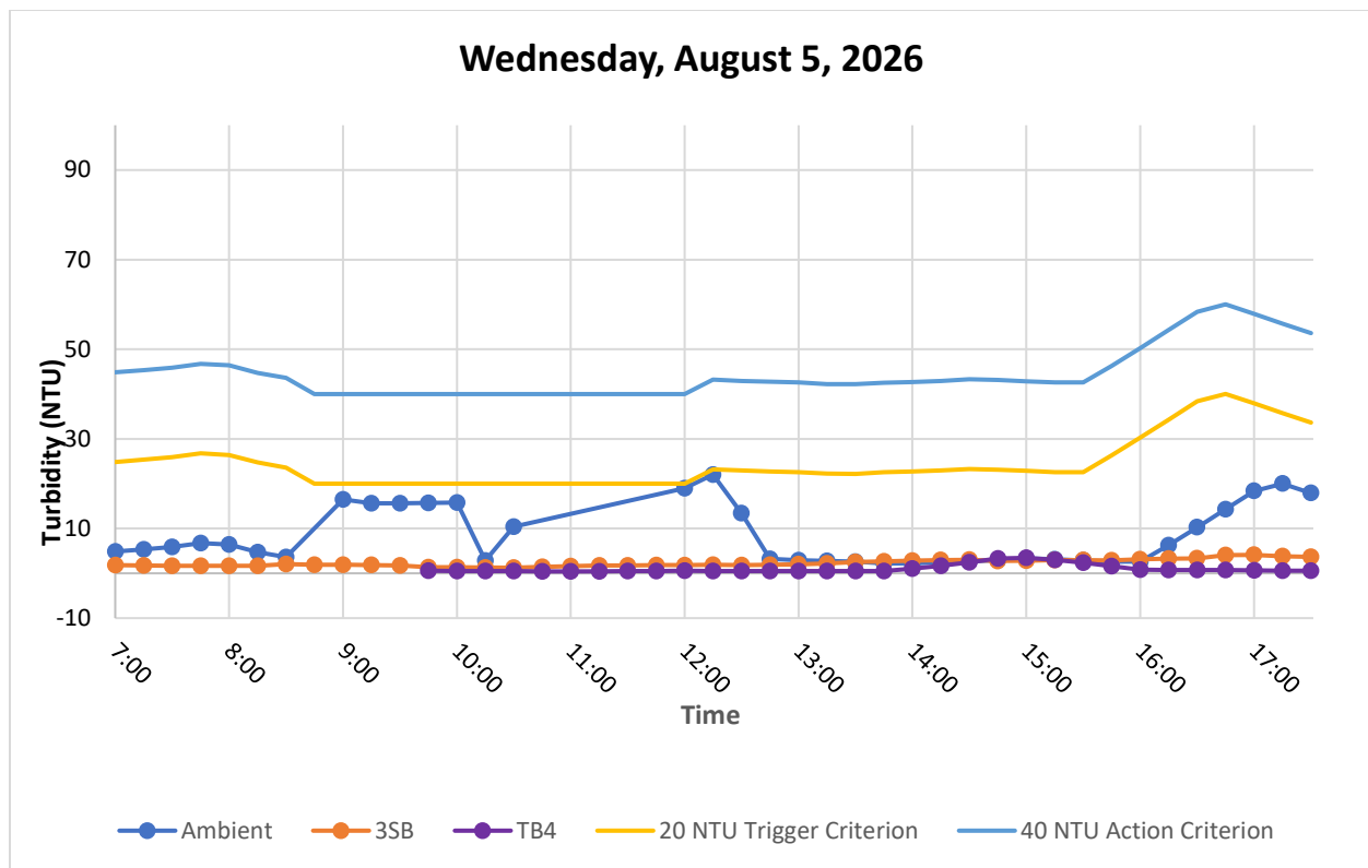
Figure 5. Hourly rolling average turbidity readings from 07:00 to 17:30.
