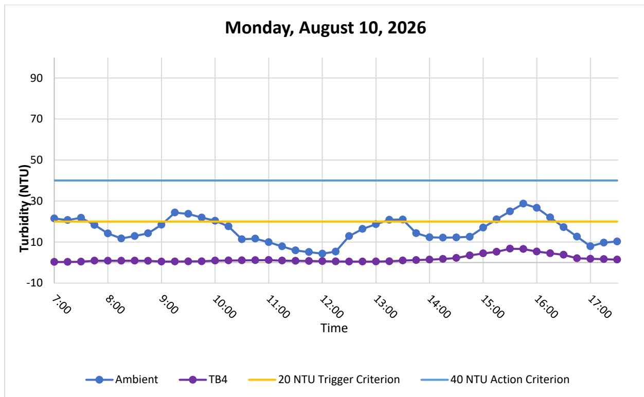
Figure 3. Hourly rolling average turbidity readings from 7:00 to 17:30.
