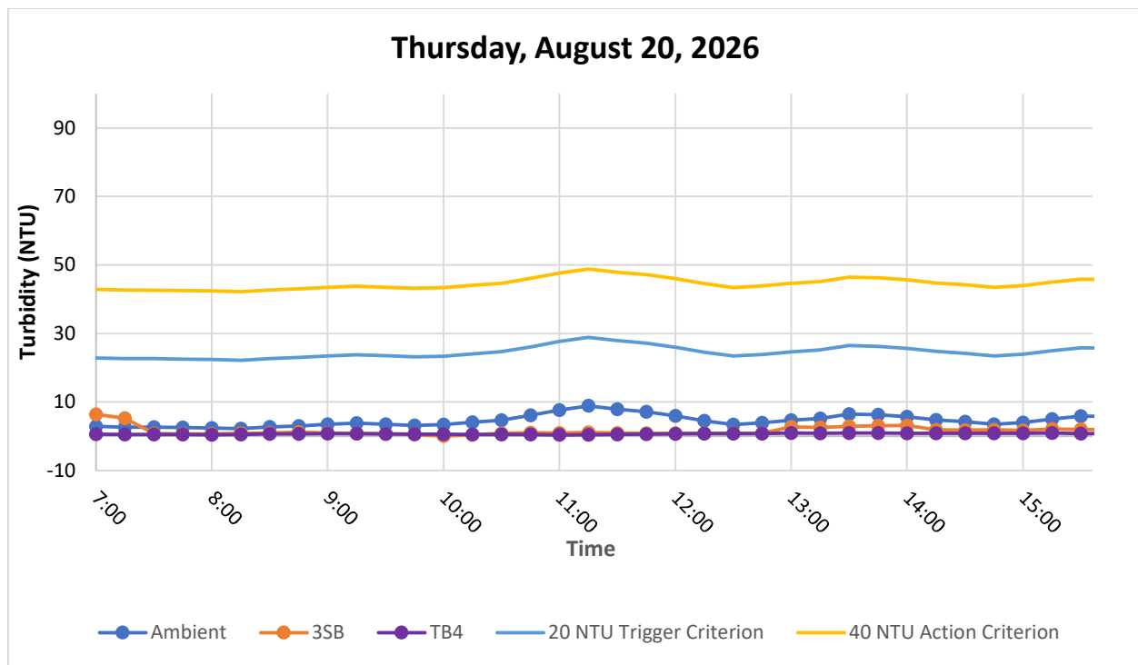
Figure 6. Hourly rolling average turbidity readings from 07:00 to 15:30.
