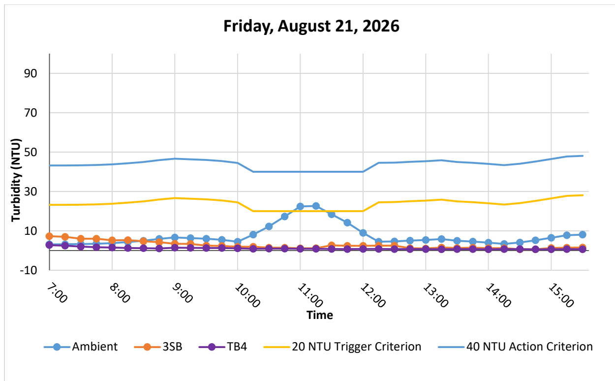
Figure 7. Hourly rolling average turbidity readings from 07:00 to 15:30. Elevated readings were not associated with in-water construction activities; see Section 3.0 for discussion.
