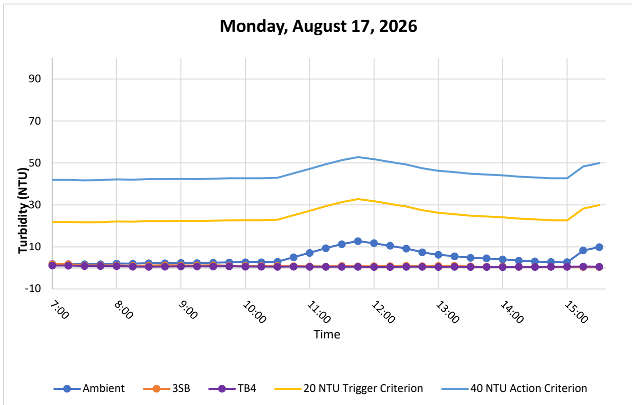
Figure 3. Hourly rolling average turbidity readings from 7:00 to 15:30.
