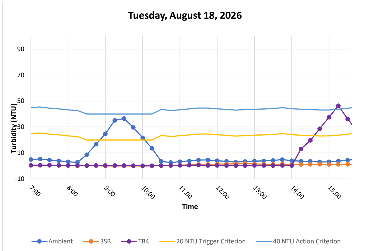
Figure 4. Hourly rolling average turbidity readings from 07:00 to 15:30. Elevated readings were not associated with in-water construction activities; see Section 3.0 for discussion.
